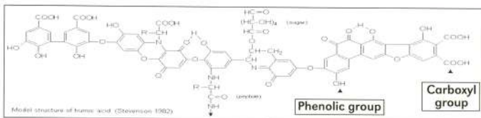
Figure 1. A simplified example of the structure of humic acid extracted from soil.
